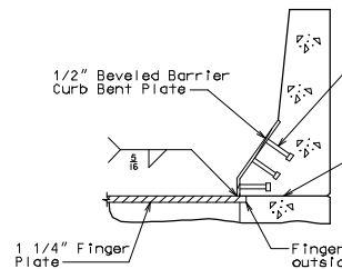
PART SECTION A-A
