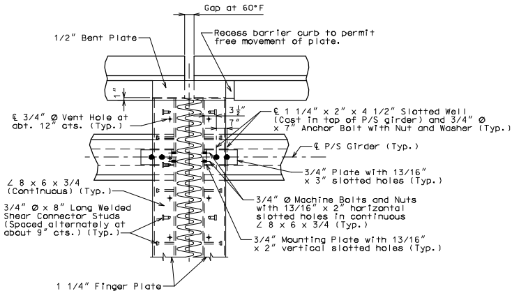
PART PLAN OF EXPANSION DEVICE
