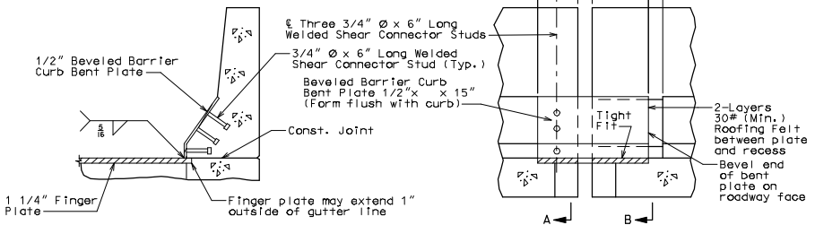
PART SECTION A-A
