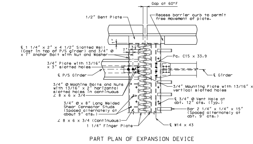
PART PLAN OF EXPANSION DEVICE
