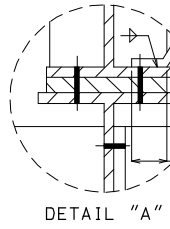
PART SECTION THRU EXPANSION DEVICE
