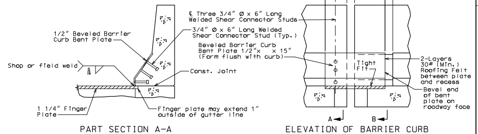
PART SECTION A-A
