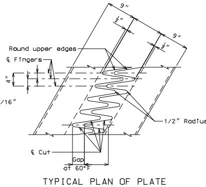
TYPICAL PLAN OF PLATE
