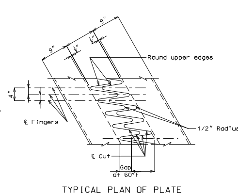
TYPICAL PLAN OF PLATE
