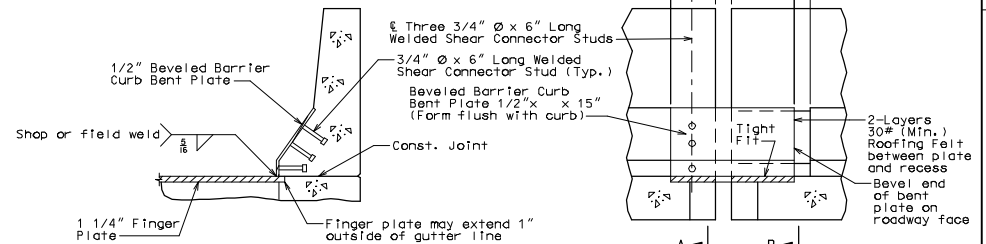
ELEVATION OF BARRIER CURB
