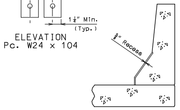
PART SECTION B-B
