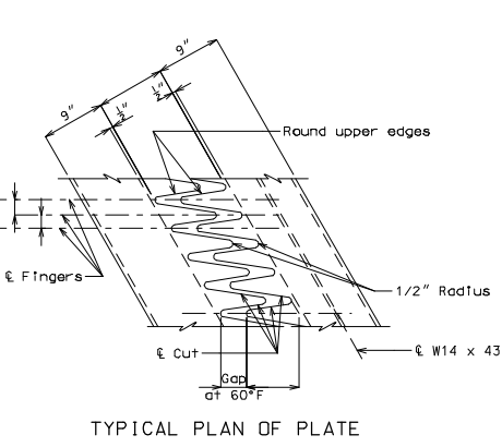
TYPICAL PLAN OF PLATE
