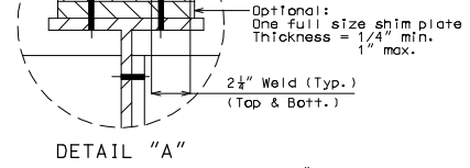
DETAIL "A"
