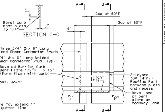
ELEVATION OF BARRIER CURB
