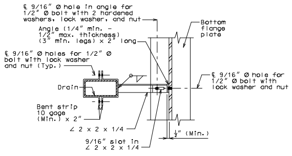
PART SECTION SHOWING BRACKET ASSEMBLY
