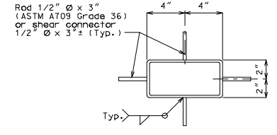
PLAN OF DRAIN
