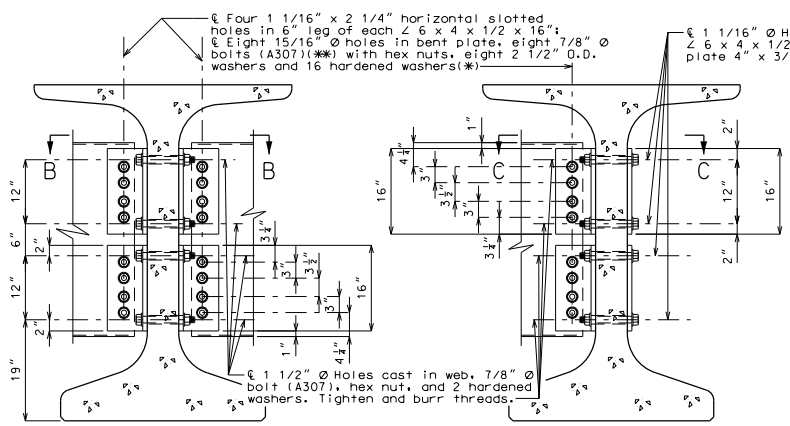
SECTION THRU INT. GIRDER AT DIAPHRAGM
