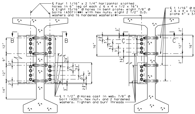
SECTION THRU INT. GIRDER AT DIAPHRAGM
