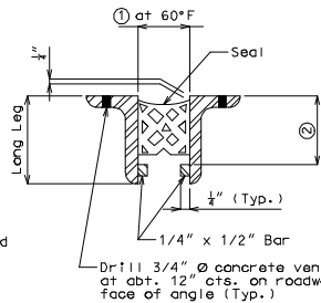
PART CROSS SECTION THRU EXPANSION JOINT
