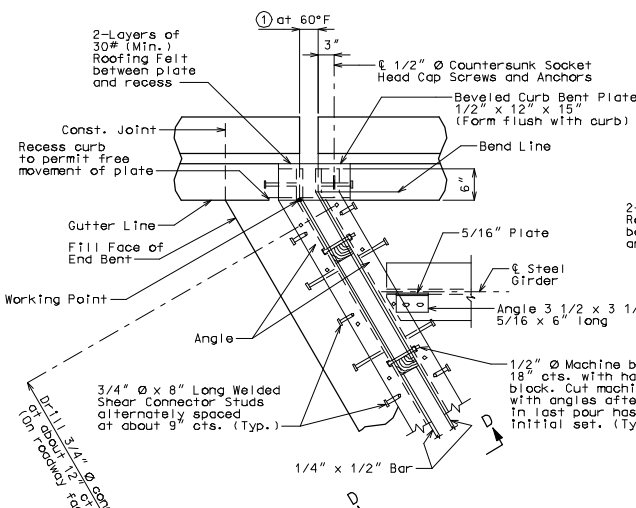
PART PLAN
