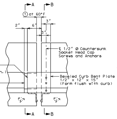
PART ELEVATION OF BARRIER CURB
