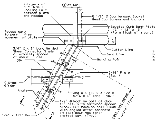
PART PLAN
