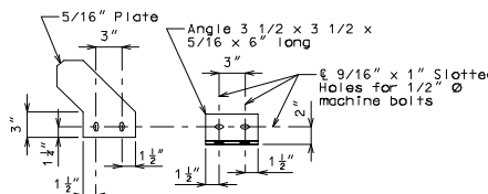
DETAIL "B"
