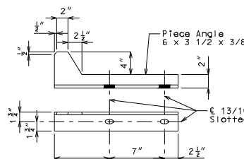
DETAIL "B"
