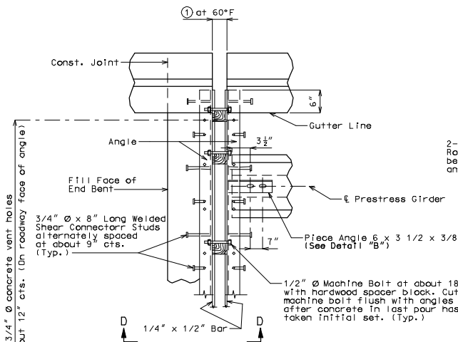
PART PLAN
