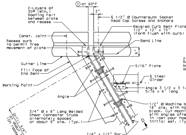
PART SECTION D-D
