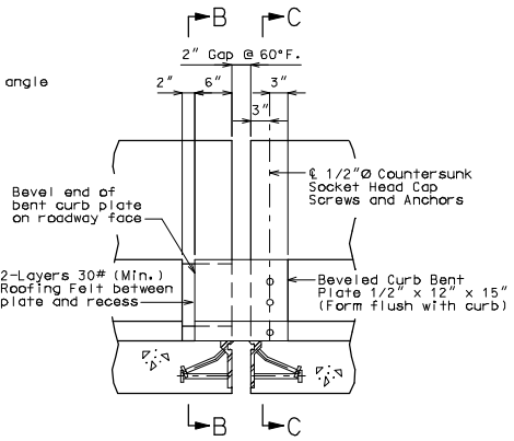
PART ELEVATION OF BARRIER CURB
