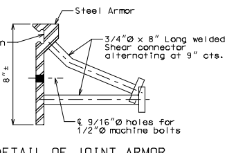
DETAIL OF JOINT ARMOR
