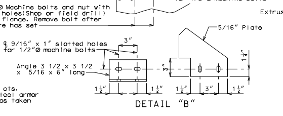
DETAIL OF JOINT ARMOR
