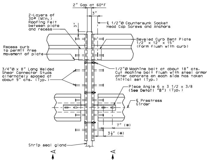
PART PLAN
