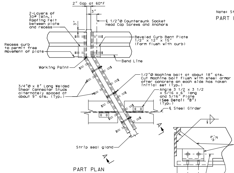
PART PLAN
