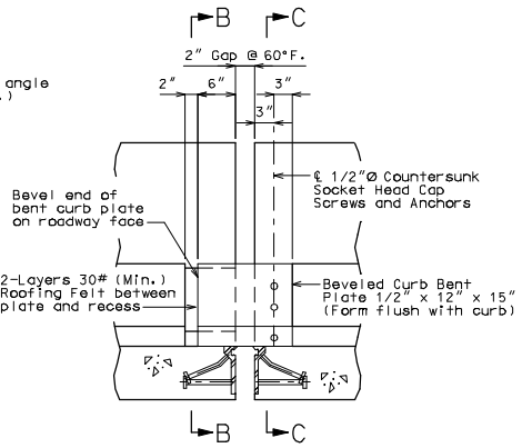
Note: Strip seal gland not shown for clarity. PART ELEVATION OF BARRIER CURB
