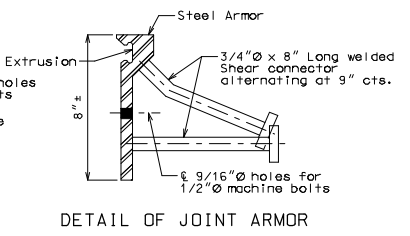
DETAIL OF JOINT ARMOR
