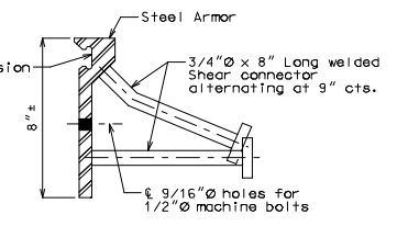
DETAIL OF JOINT ARMOR
