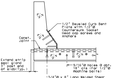
PART SECTION C-C
