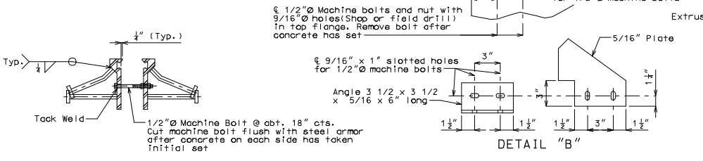
DETAILS OF STRIP SEAL AT END BENT NO.
