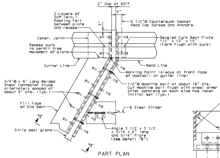
PART PLAN
