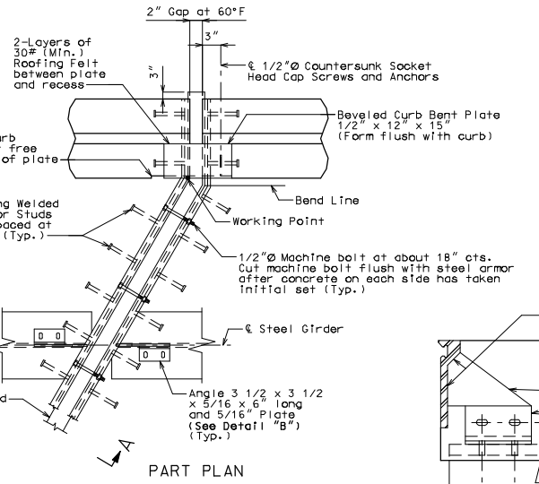
PART PLAN
