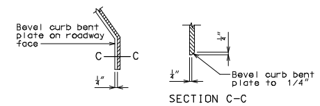
SECTION C-C
