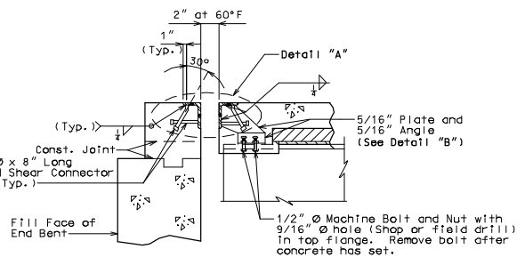
PART SECTION D-D
