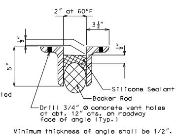
PART CROSS SECTION THROUGH EXPANSION JOINT
