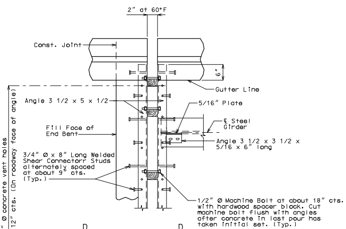
PART PLAN
