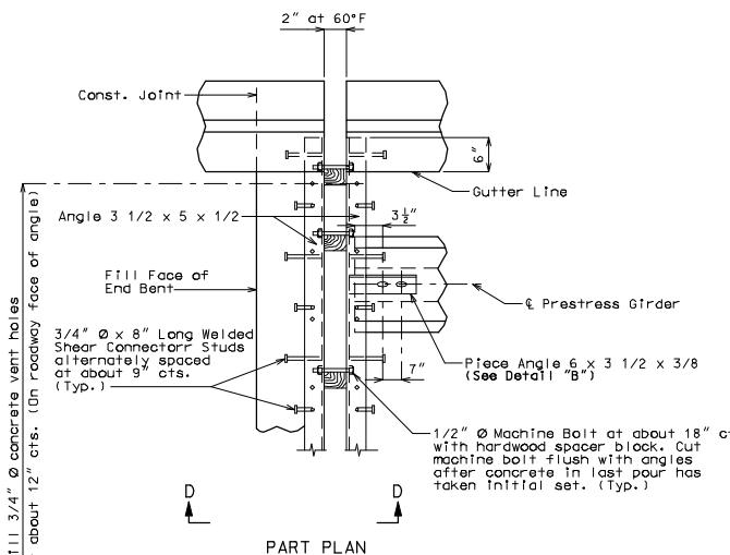
PART PLAN
