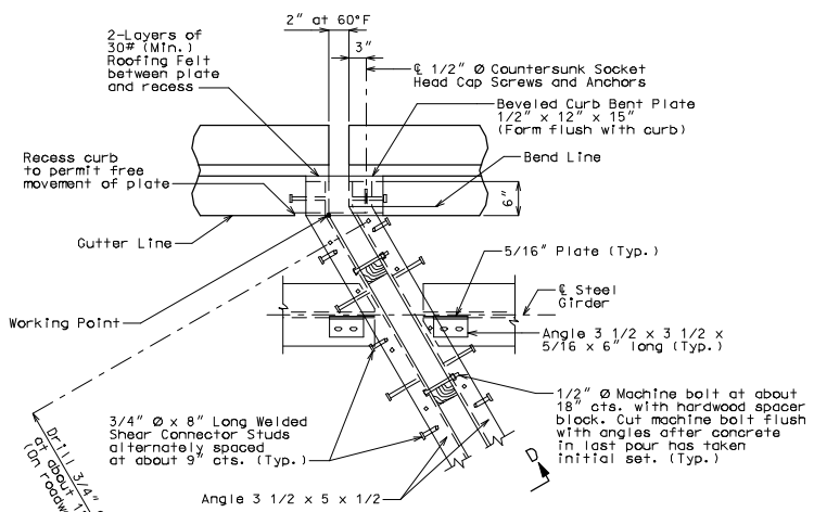
PART PLAN
