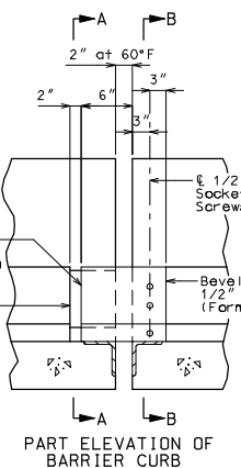
PART ELEVATION OF BARRIER CURB
