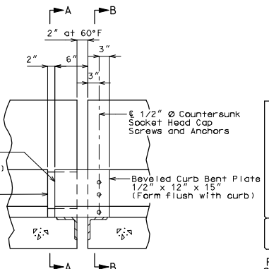
PART ELEVATION OF BARRIER CURB
