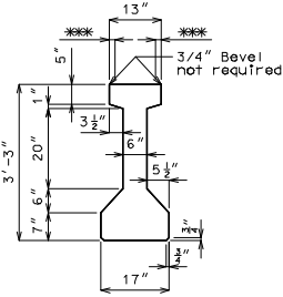
GIRDER DIMENSIONS
