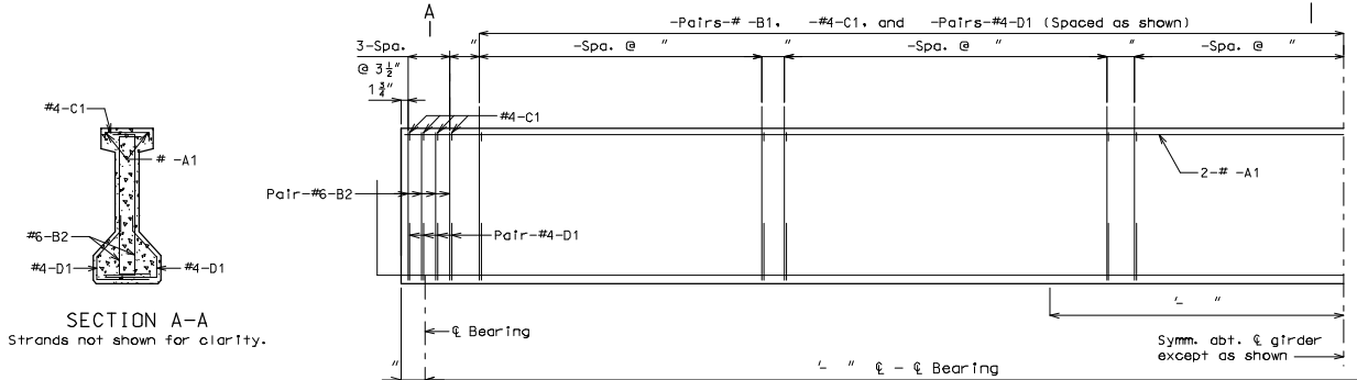
HALF ELEVATION OF GIRDER SPAN ( - )
