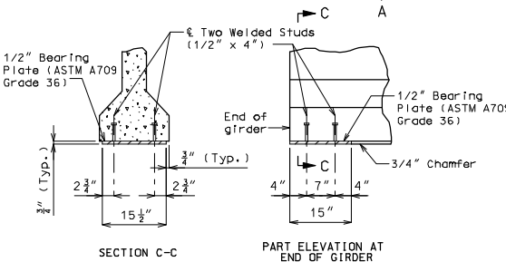
SECTION C-C BEARING PLATE DETAILS
