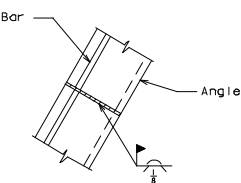
PART PLAN OF ANGLE AND BAR
