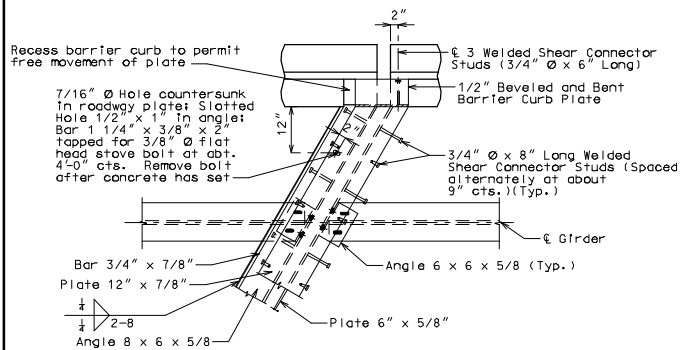
PART PLAN
