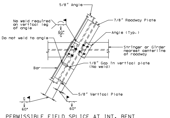
PERMISSIBLE FIELD SPLICE AT INT. BENT
