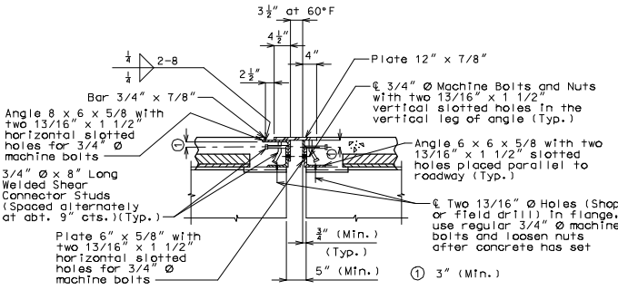
PART SECTION AT INTERMEDIATE BENT
