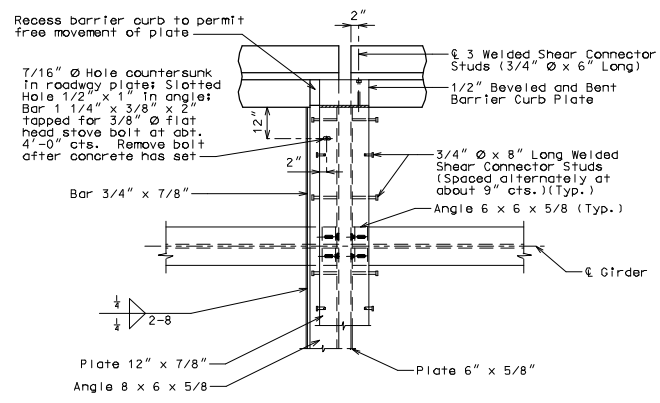
PART PLAN
