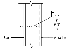
PART PLAN OF ANGLE AND BAR
