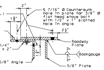
PART SECTION (TYPICAL)
