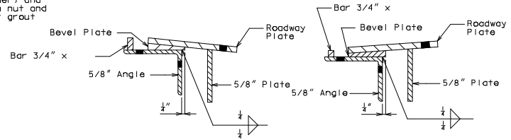
PART SECTION THRU BEVEL PLATE
