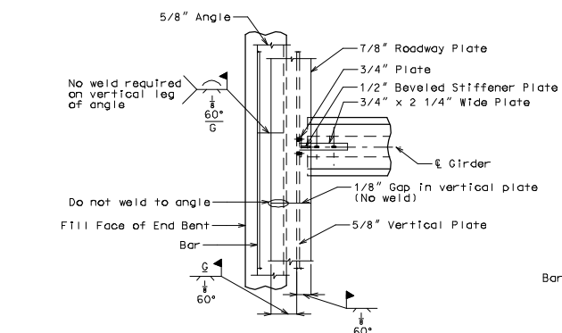
PERMISSIBLE FIELD SPLICE AT END BENT
