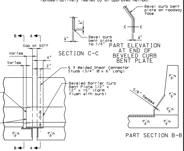
ELEVATION OF BARRIER CURB
