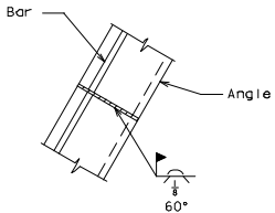
PART PLAN OF ANGLE AND BAR
