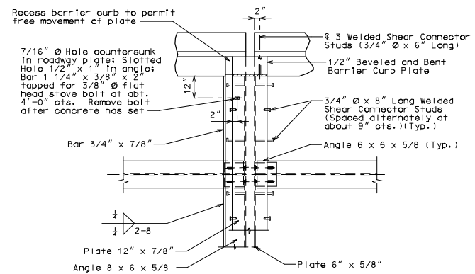
PART PLAN
