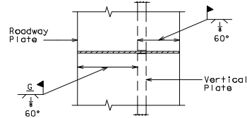
PART PLAN ROADWAY PLATE AND VERTICAL PLATE
