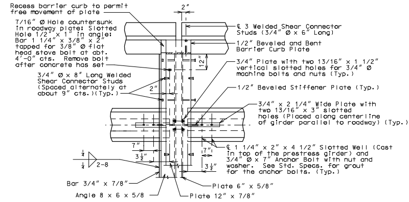
PART PLAN
