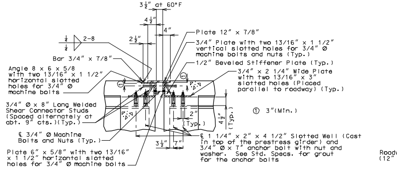
PART SECTION AT INTERMEDIATE BENT
