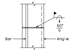
PART PLAN OF ANGLE AND BAR
