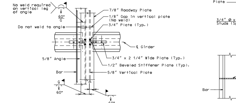
PART PLAN OF ANGLE AND BAR
