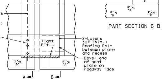
ELEVATION OF BARRIER CURB
