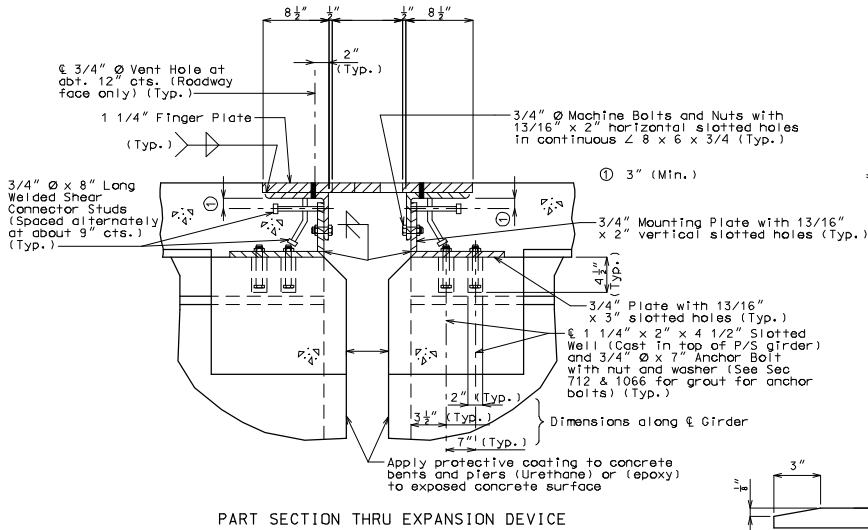
PART SECTION THRU EXPANSION DEVICE
