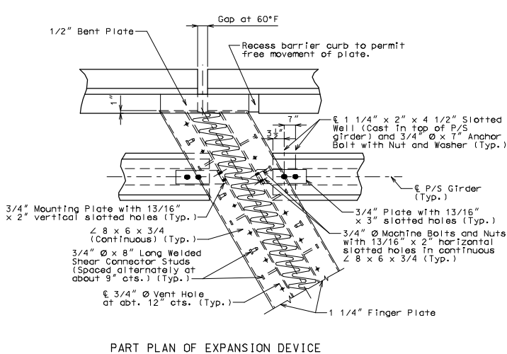
PART PLAN OF EXPANSION DEVICE
