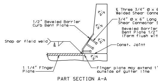
PART SECTION A-A
