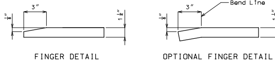
FINGER DETAIL
