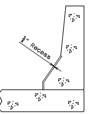
PART SECTION B-B
