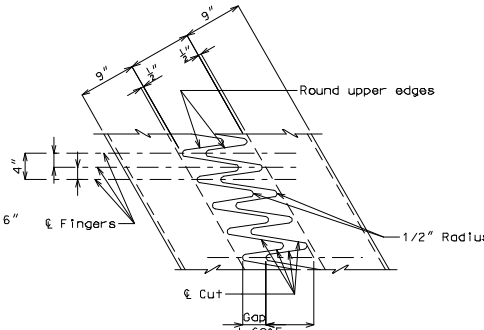
TYPICAL PLAN OF PLATE
