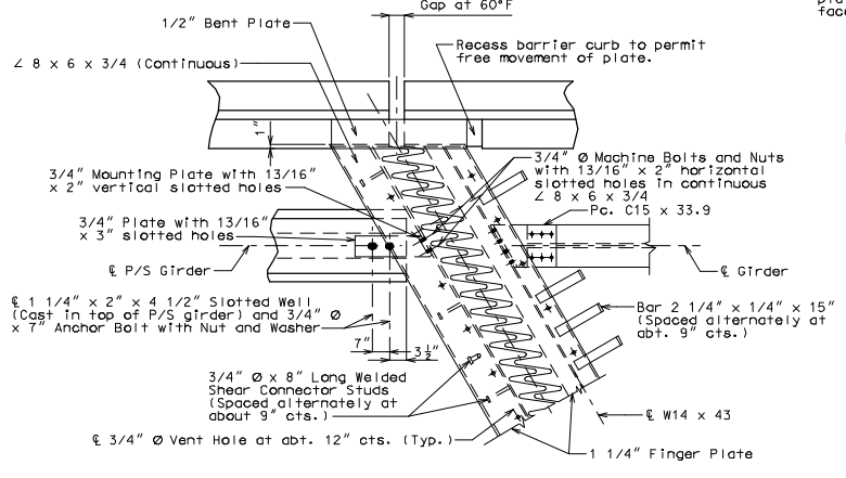
PART PLAN OF EXPANSION DEVICE
