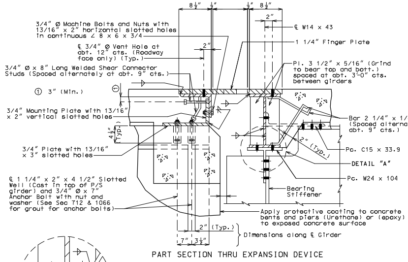
PART SECTION THRU EXPANSION DEVICE
