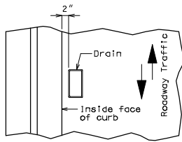
PART SECTION NEAR DRAIN
