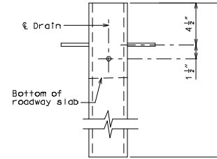
ELEVATION OF DRAIN
