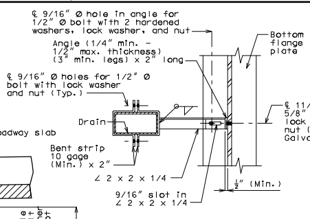
PART SECTION SHOWING BRACKET ASSEMBLY
