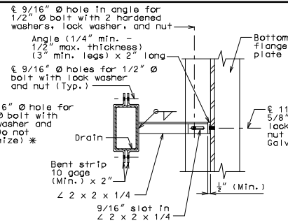
PART SECTION SHOWING BRACKET ASSEMBLY
