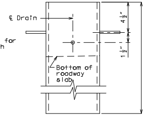
ELEVATION OF DRAIN
