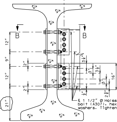
SECTION THRU INT. GIRDER AT DIAPHRAGM
