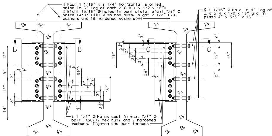
SECTION THRU INT. GIRDER AT DIAPHRAGM
