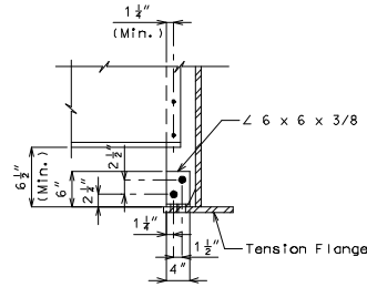
DETAIL "D"
