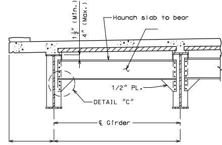
TYPICAL PART SECTION SHOWING END DIAPHRAGMS
