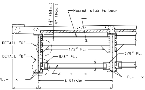
TYPICAL PART SECTION SHOWING END DIAPHRAGMS
