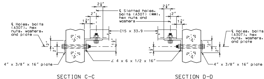
SECTION C-C
