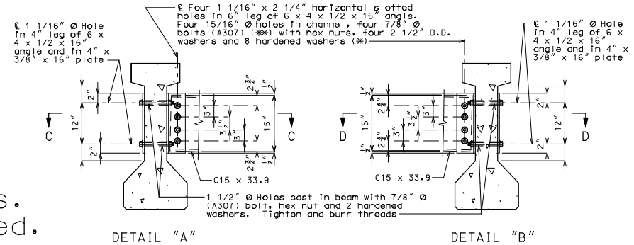
DETAIL "A"
