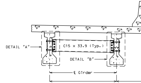
PART SECTION SHOWING INTERMEDIATE DIAPHRAGMS
