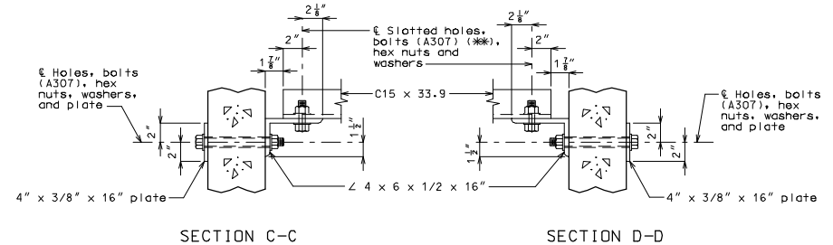
SECTION C-C
