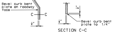
SECTION C-C PART ELEVATION AT END OF BEVELED CURB BENT PLATE
