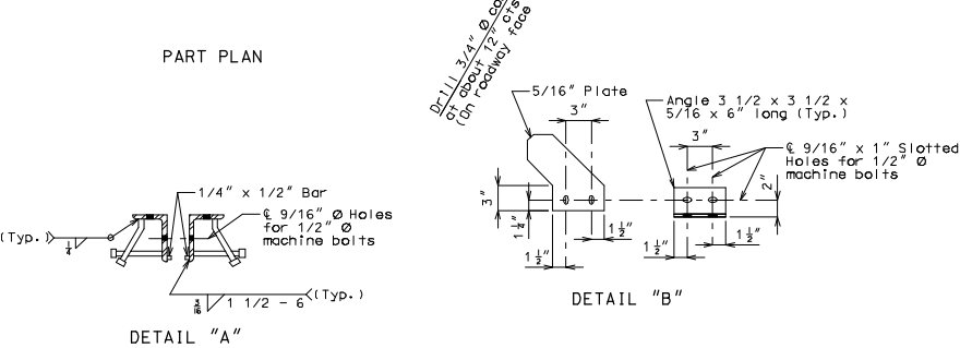
DETAILS OF PREFORMED COMPRESSION JOINT SEAL AT INT. BENT NO.
