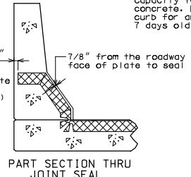
PART SECTION THRU JUNCTION SEAL
