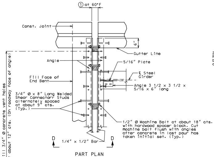
PART PLAN
