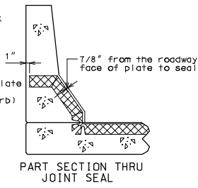
PART SECTION THRU JOINT SEAL
