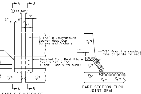
PART ELEVATION OF BARRIER CURB
