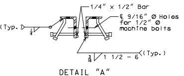
DETAIL "A"
