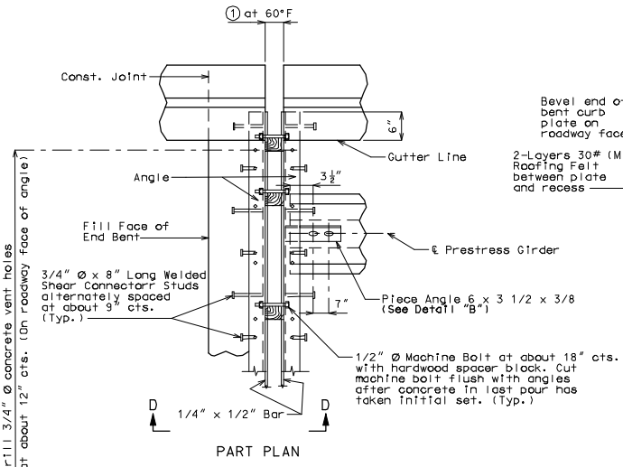
PART PLAN
