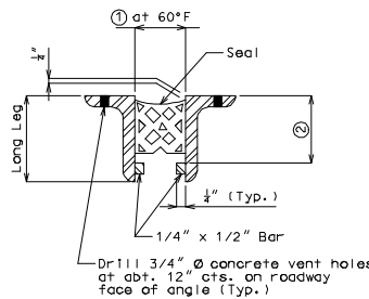
PART CROSS SECTION THRU JOINT SEAL
