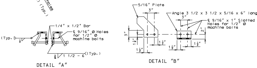
DETAIL "A"
