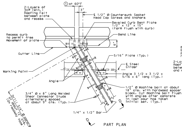
PART PLAN
