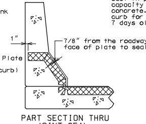
PART SECTION THRU JOINT SEAL
